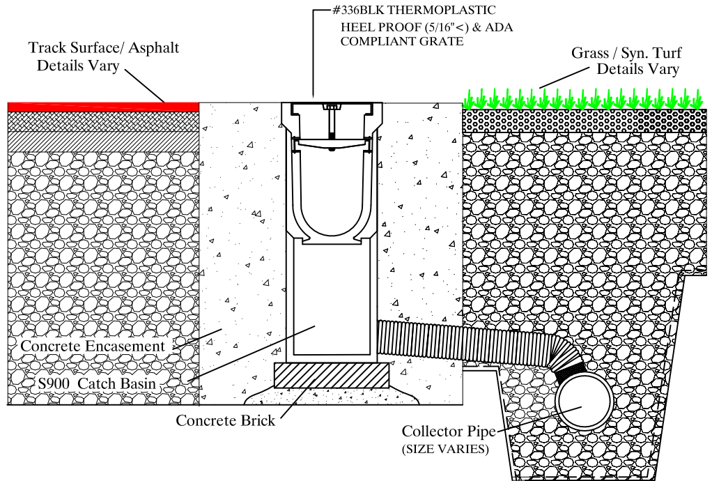
SPORTSEGE 900 Catch Basin NO SCALE End View
