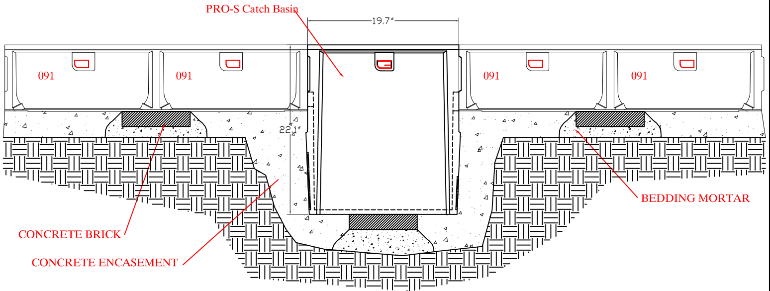
S900 In Line Catch Basin - Side View
