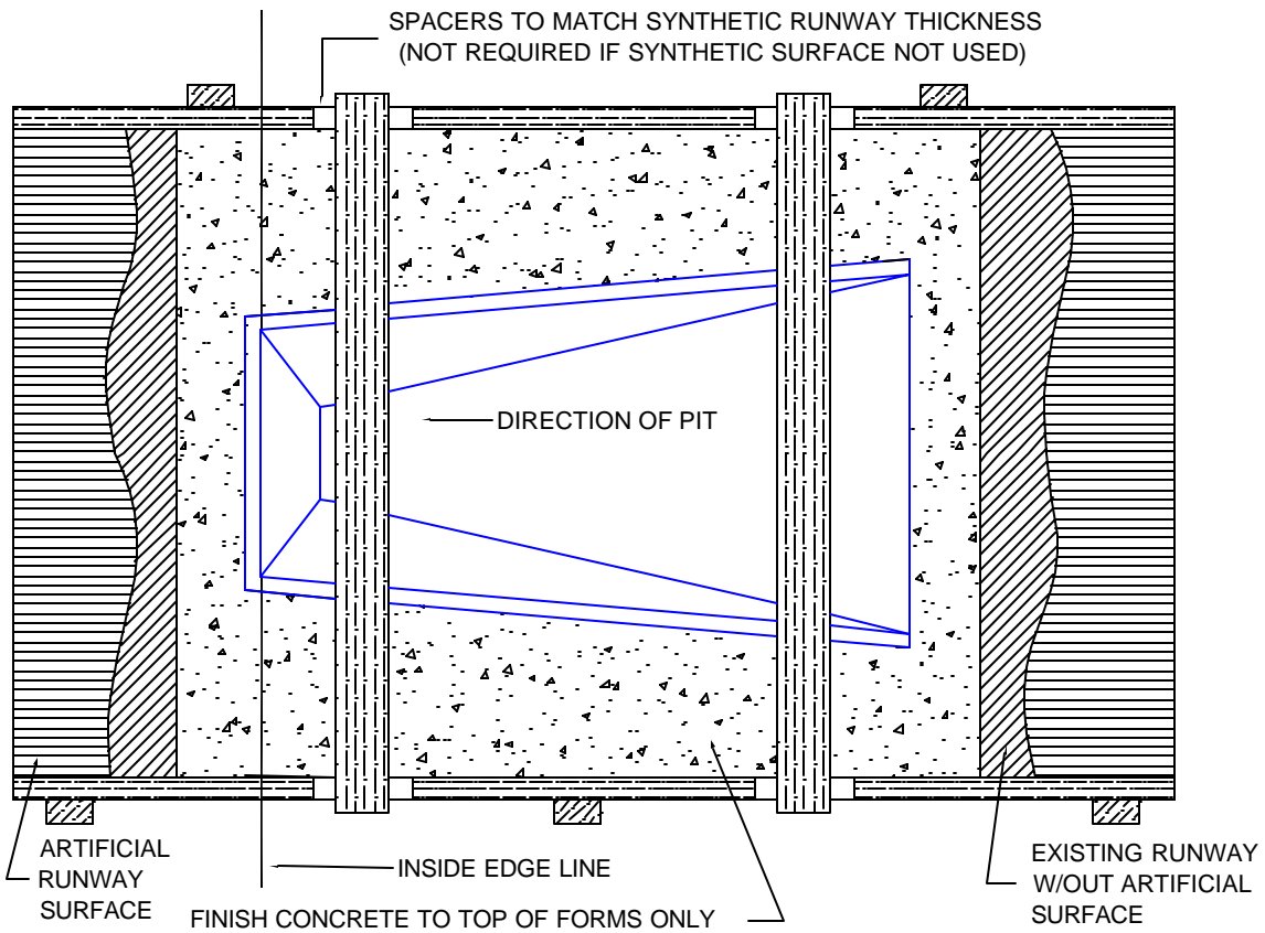
PLAN VIEW FOLLOWING CONCRETE POUR
