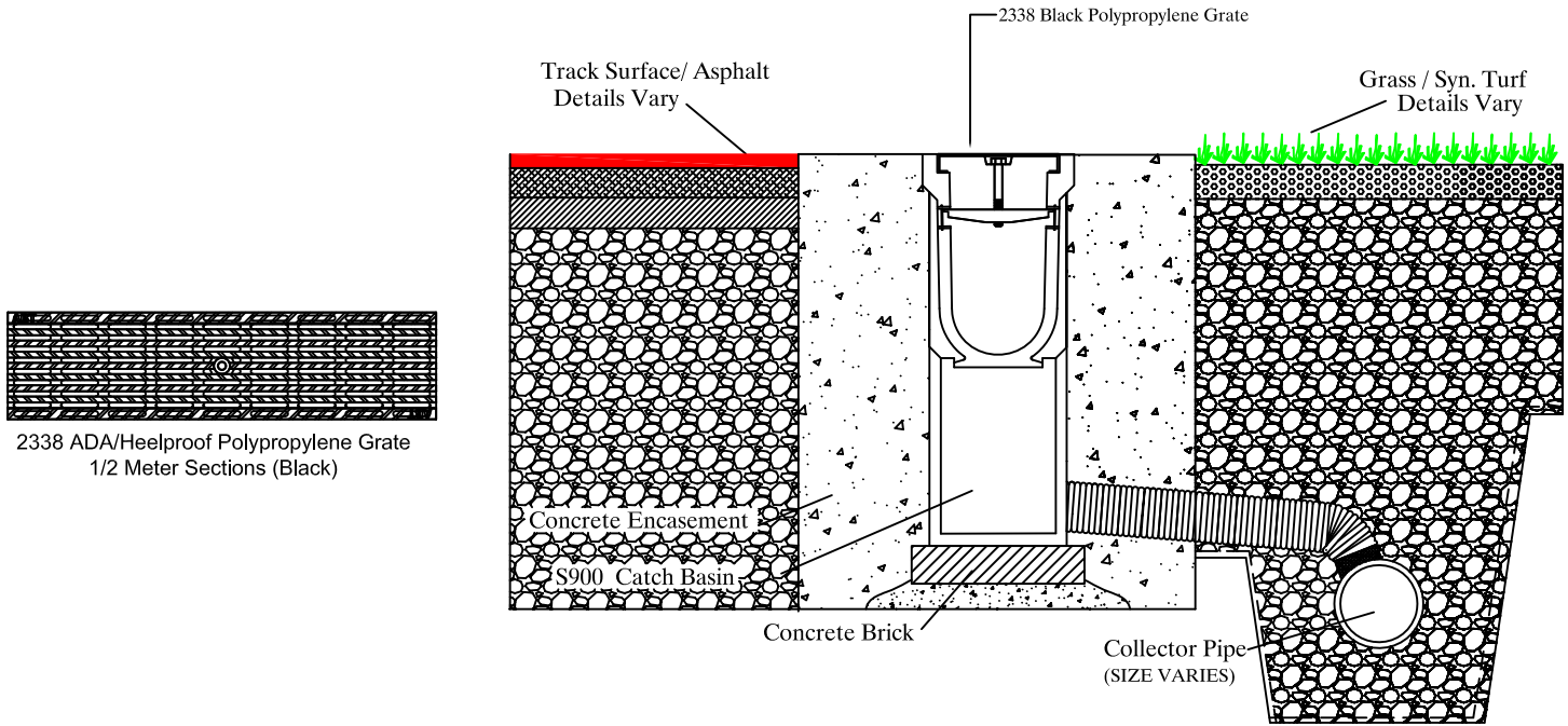
SPORTSEGE 900 Catch Basin NO SCALE End View
