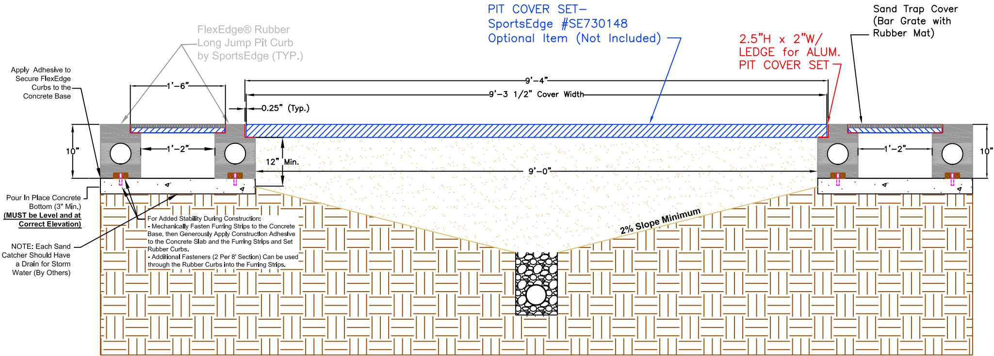
SECTION FlexEdge Rubber Long Jump Pit Curbs w/ Sand catchers and Pit Cover Set
