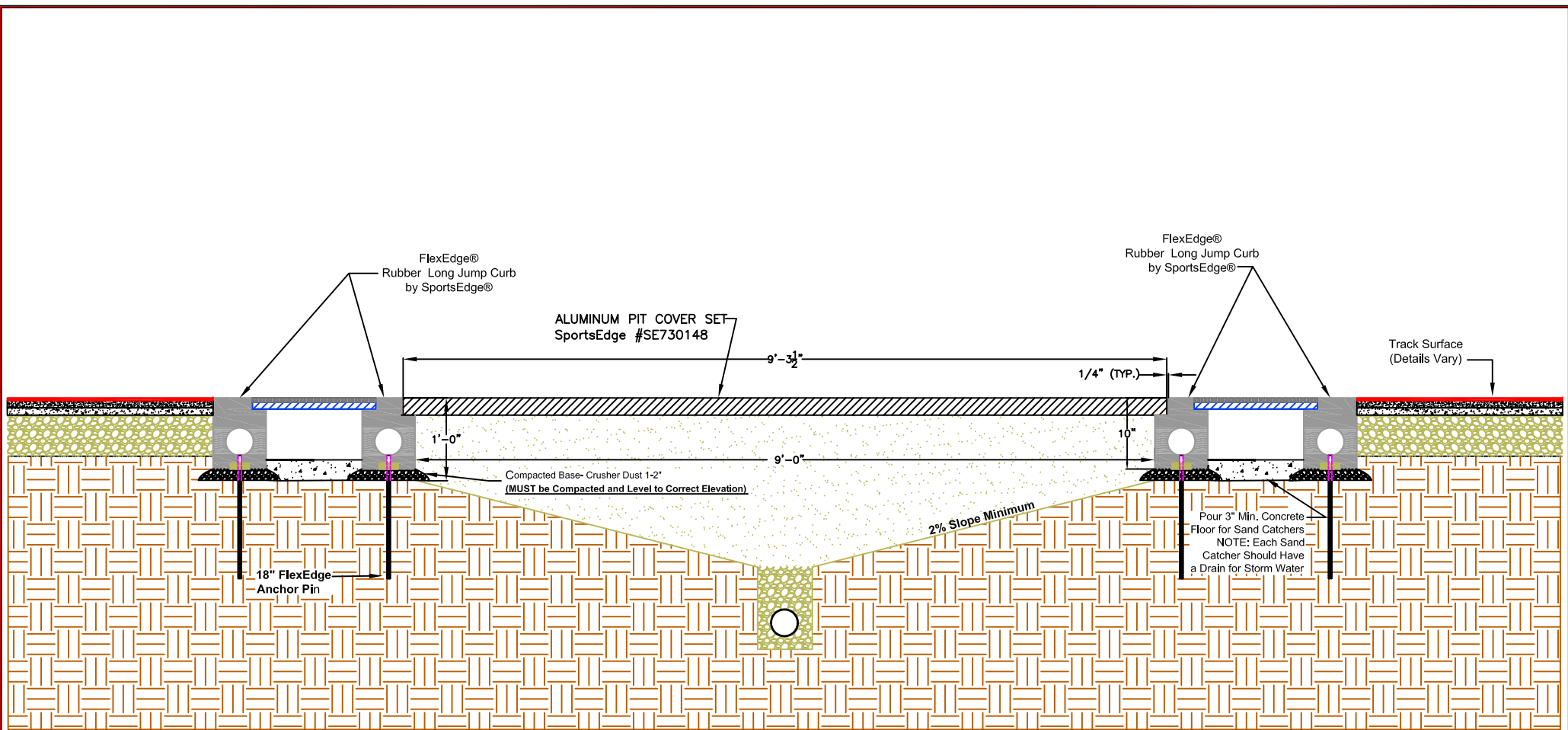
SECTION - Synthetic Turf to FlexEdge Long Jump Pit w/ Sand catchers and Pit Cover Set - Option 2
