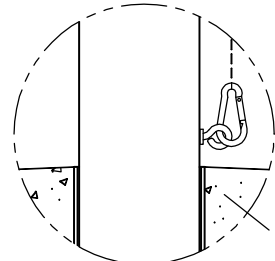
Eyebolt & Spring Snap Anchor Net at Bottom of Pole
