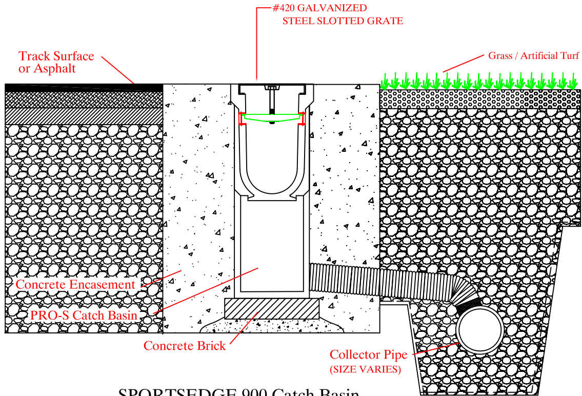
SPORTSEGE 900 Catch Basin NO SCALE End View
