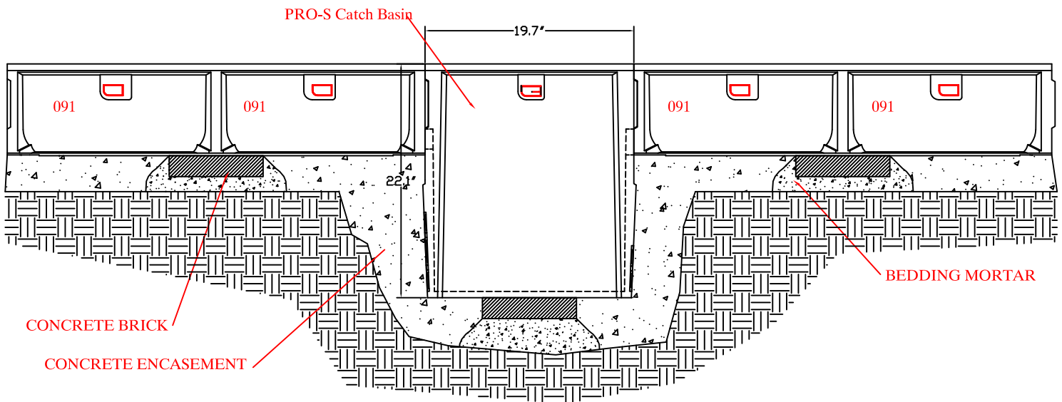
900 In Line Catch Basin NO SCALE Side View
