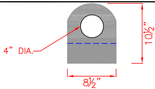
END PROFILE
