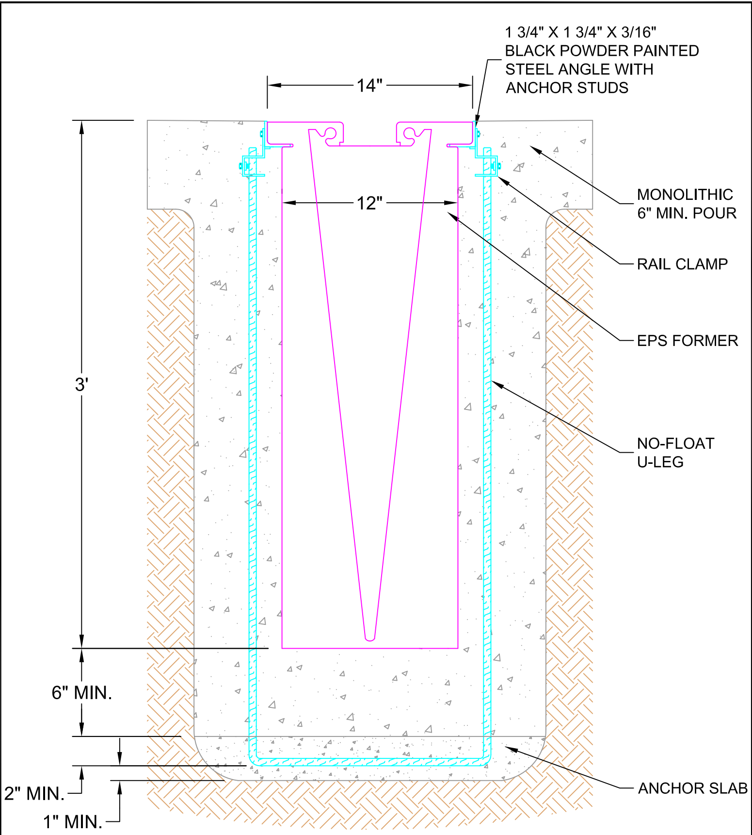
END CROSS SECTION VIEW
