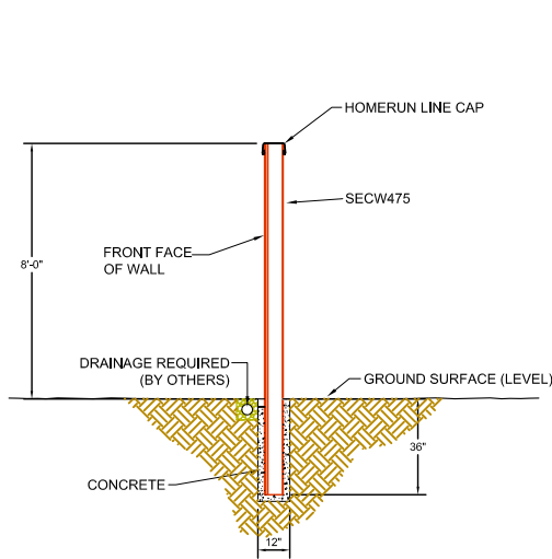
TYPICAL CROSS-SECTION 8 FT. WALL
