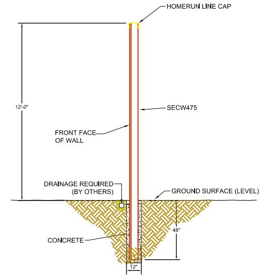
TYPICAL CROSS-SECTION 12 FT. WALL
