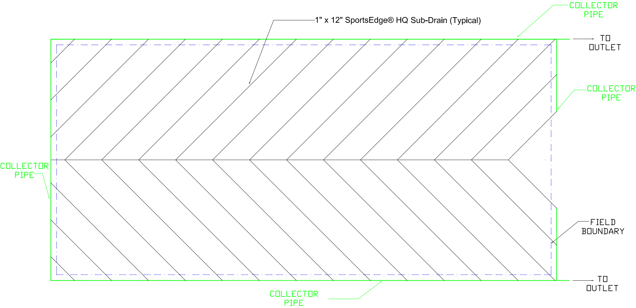
TYPICAL DRAINAGE LAYOUT - SportsEdge® HQ-12 ATHLETIC FIELD INSTALLATION
