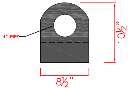
END PROFILE
