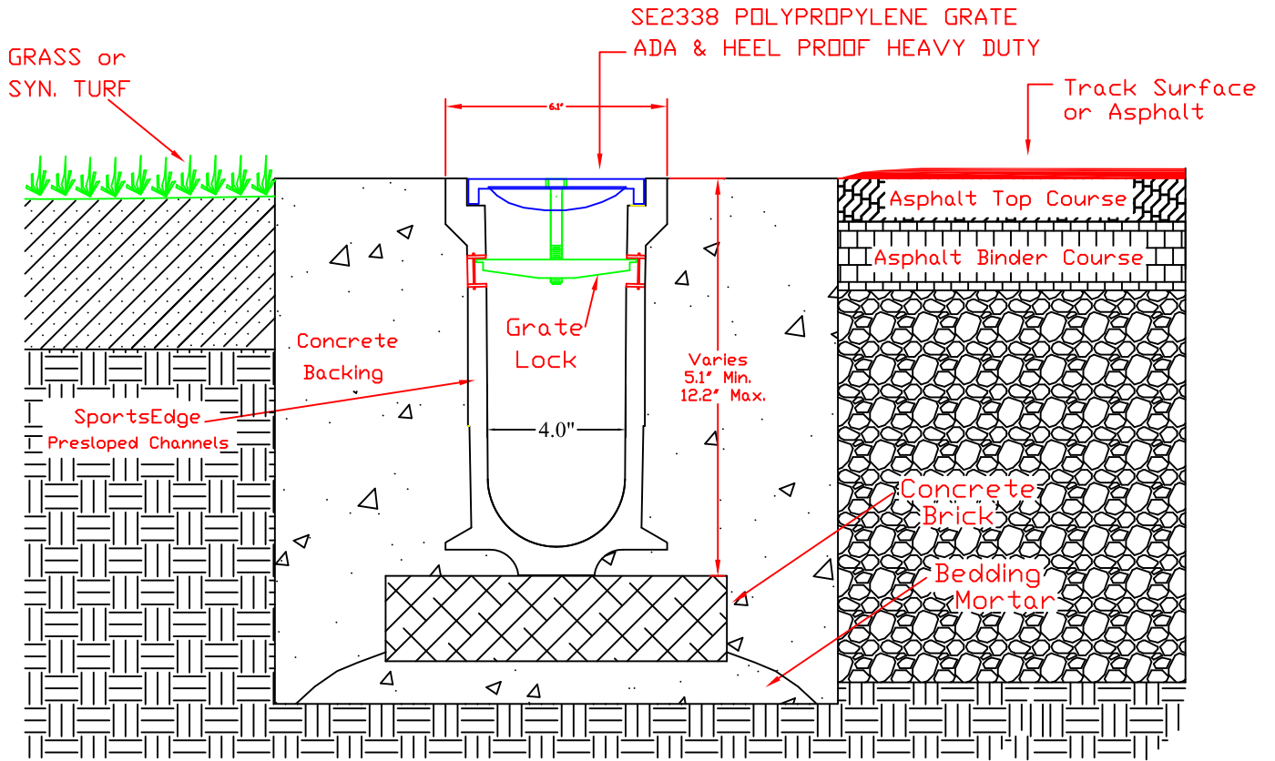
SportsEdge SE2338 with Presloped PolyDrain NO SCALE
