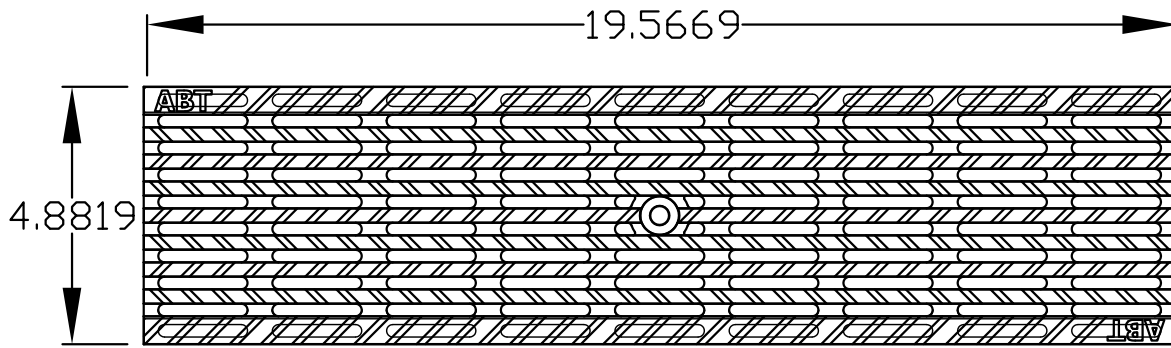
2338 ADA/Heelproof Polypropylene Grate 1/2 Meter Sections (Black)
