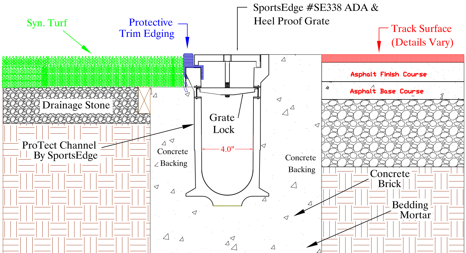
SportsEdge ProProtect Channel - S192M Channel Drain Protective Trim Edge One Side NO SCALE
