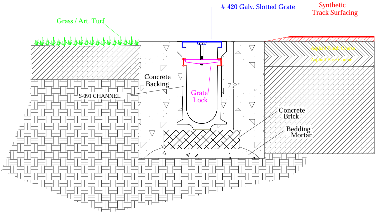
Section- SportsEdge Pro-S Channel #S-091 Typ. Detail- No Scale
