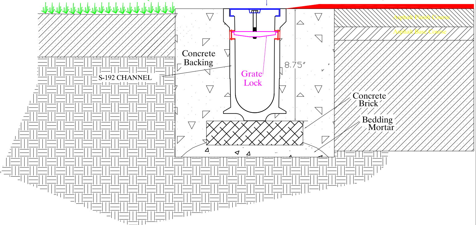
Section- SportsEdge Pro-S Channel #S-192 Typ. Detail- No Scale - Option 2
