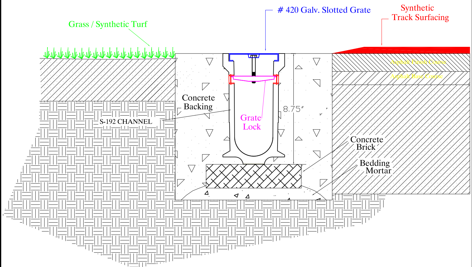
Section- SportsEdge Pro-S Channel #S-192 Typ. Detail- No Scale
