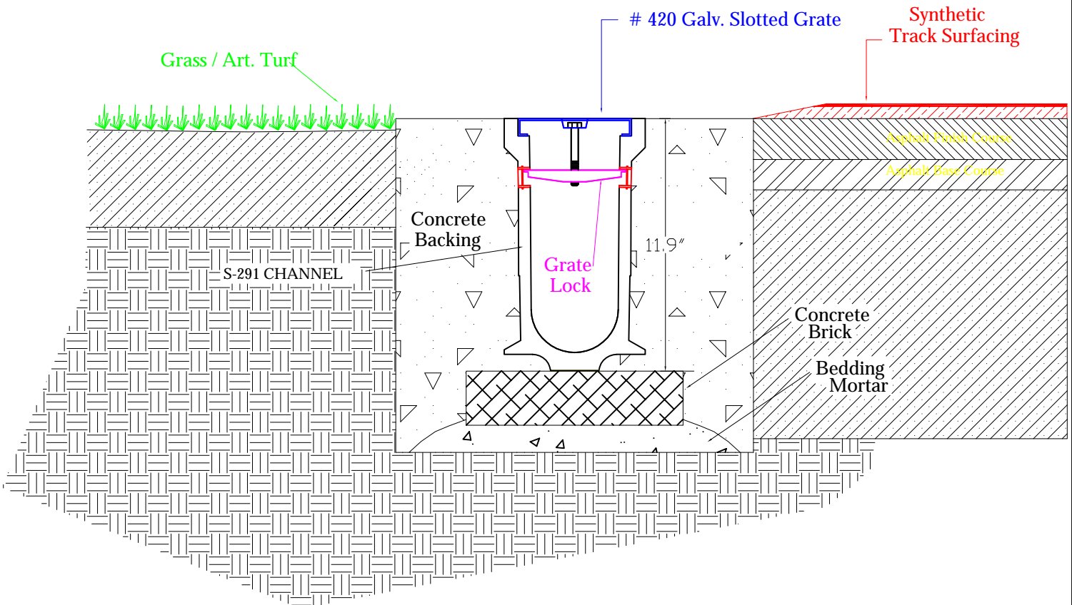
Section- SportsEdge Pro-S Channel #S-291 Typ. Detail- No Scale
