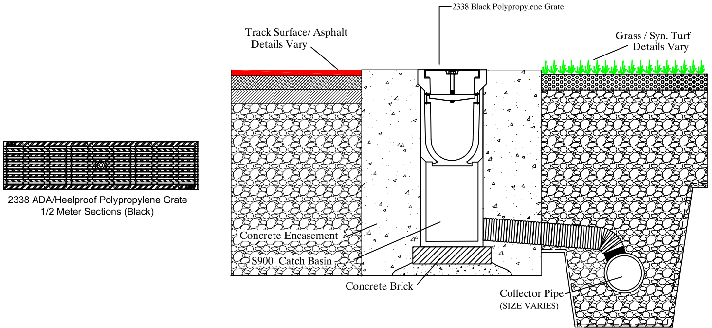
SPORTSEdge 900 Catch Basin NO SCALE End View
