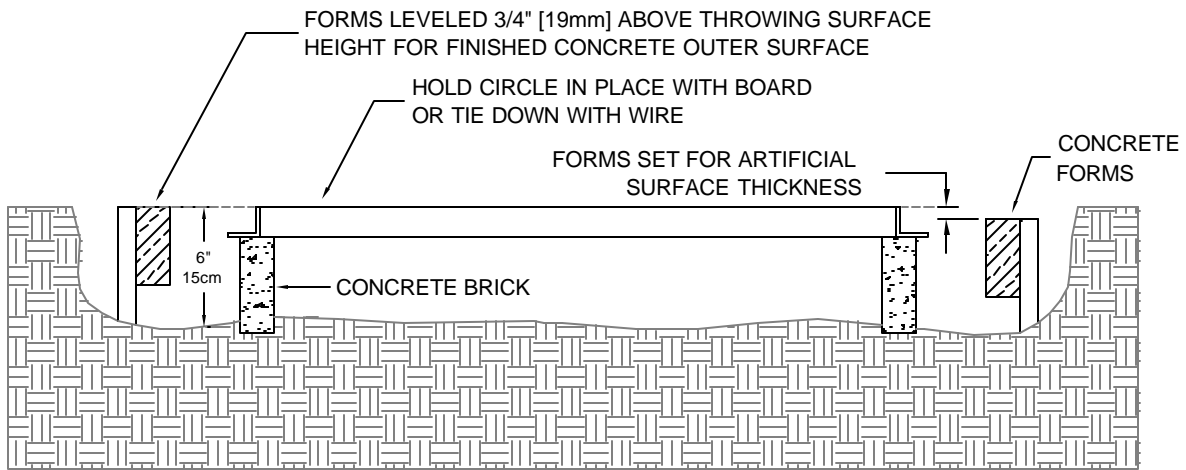
SECTION A-A #1
