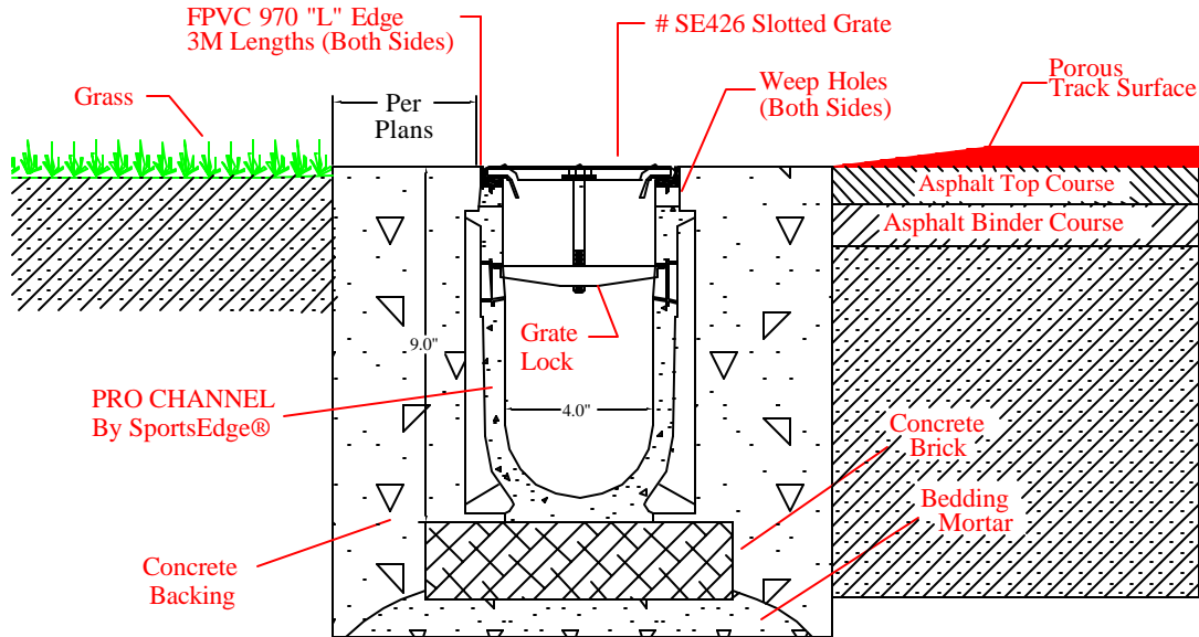
SE426 SPORTSEGE® PRO Channel Drain - 2 Curb Application
