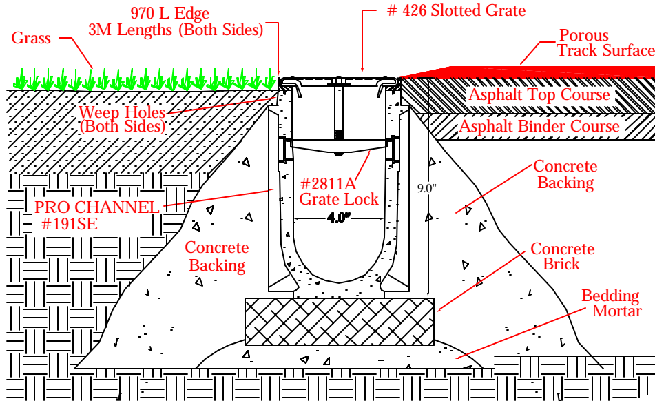
SE426 SPORTSEGE® PRO Channel Drain - No Curb Application
