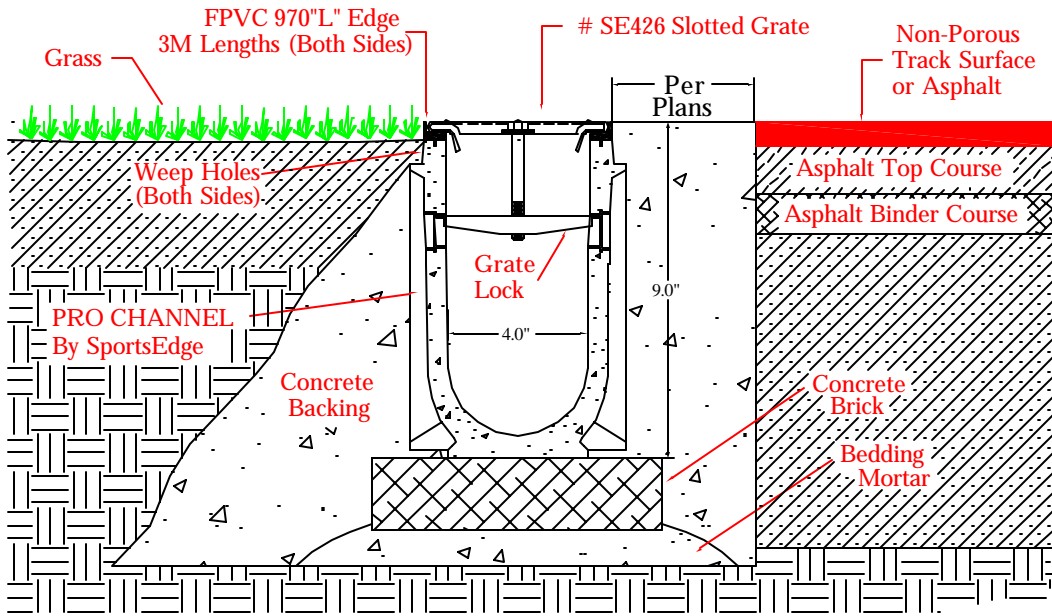
SE426 SPORTSEGE® PRO Channel Drain - 1 Side Curb Application
