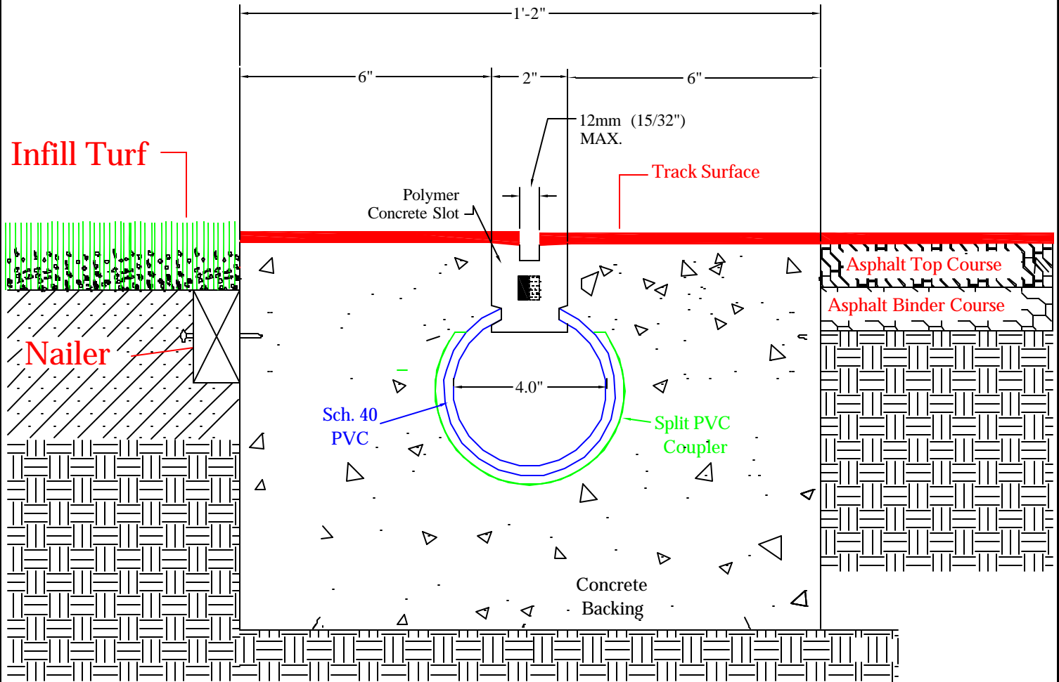
SPORTSEdge® XT Slot Drain - Infill Turf w/ Nailer NO SCALE
