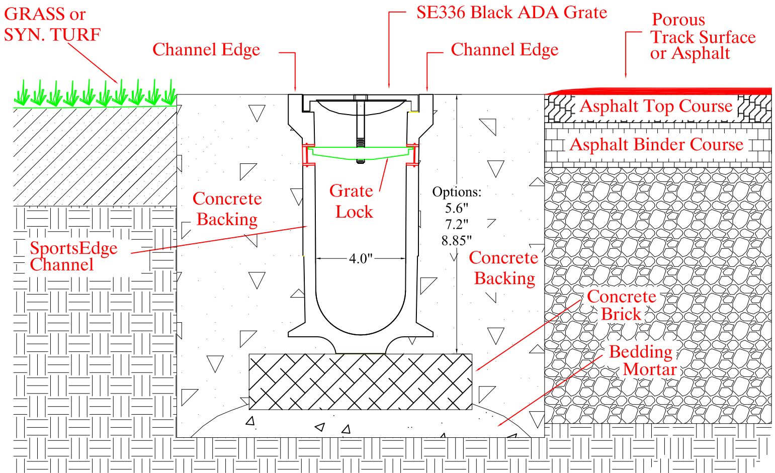
SPORTSEGE SE336 Channel Drain - 2 Curb Application Porous Track Surface or Asphalt NO SCALE
