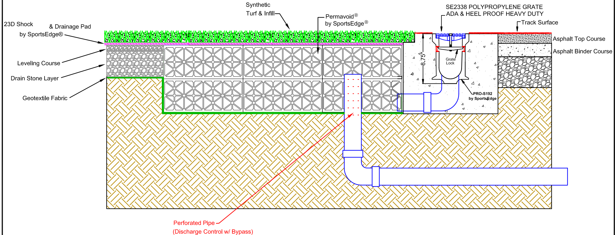
Plan View- SportsEdge PRO-S192 Surface Drain System w/ 23D Shock/Drain Pad and Permavoid Water Control System
