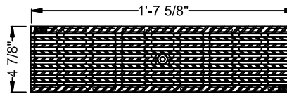
PLAN VIEW
