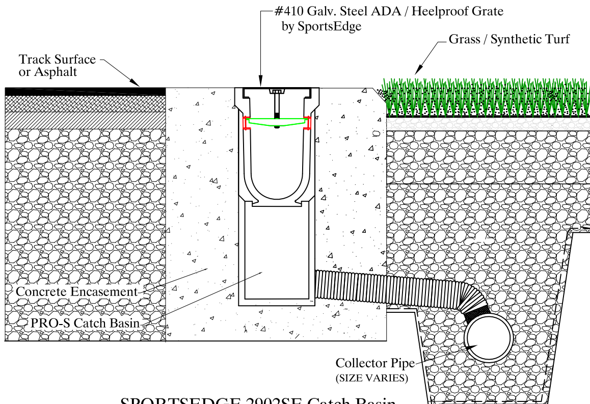
SPORTSEGE 2902SE Catch Basin NO SCALE End View
