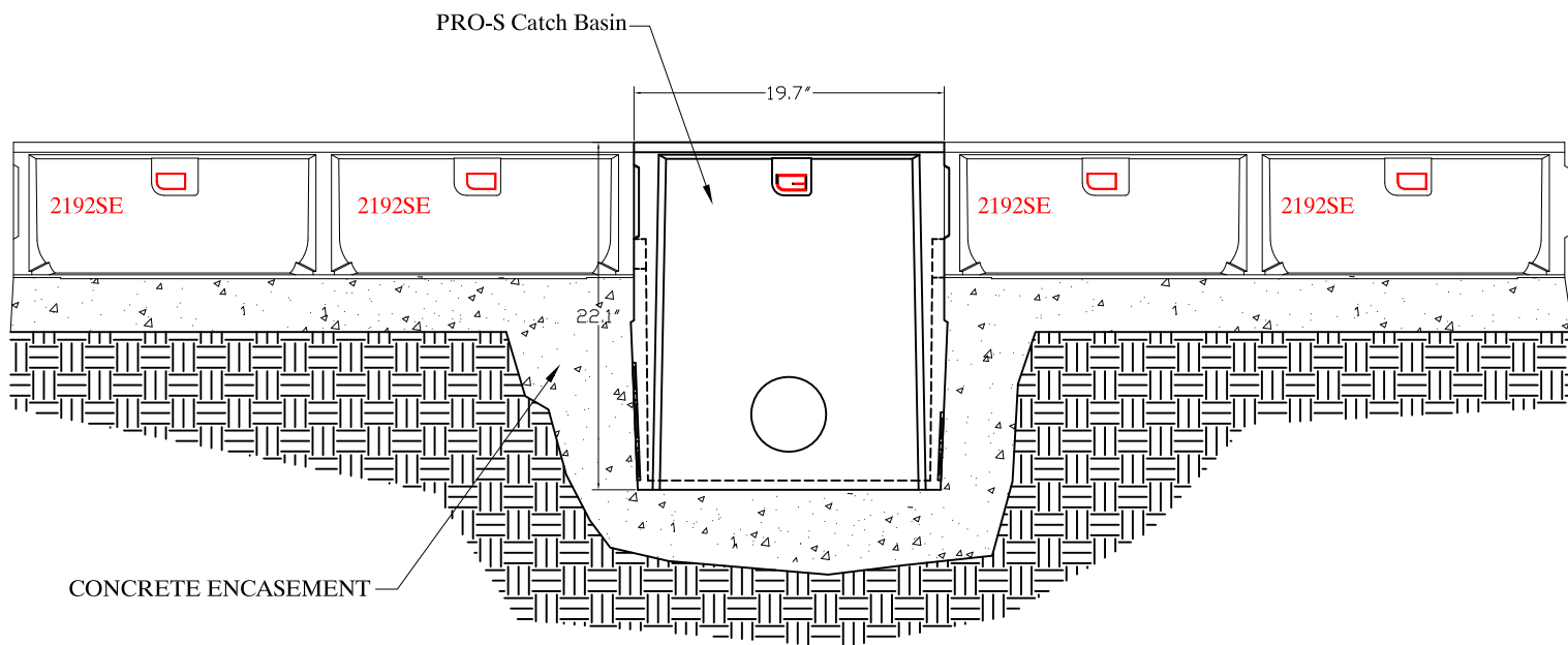
2902SE In Line Catch Basin NO SCALE Side View
