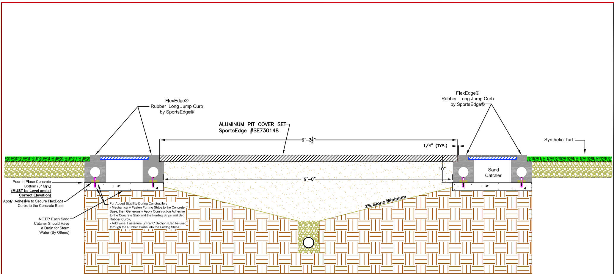
SECTION - Synthetic Turf to FlexEdge Long Jump Pit w/ Sand catchers and Pit Cover Set
