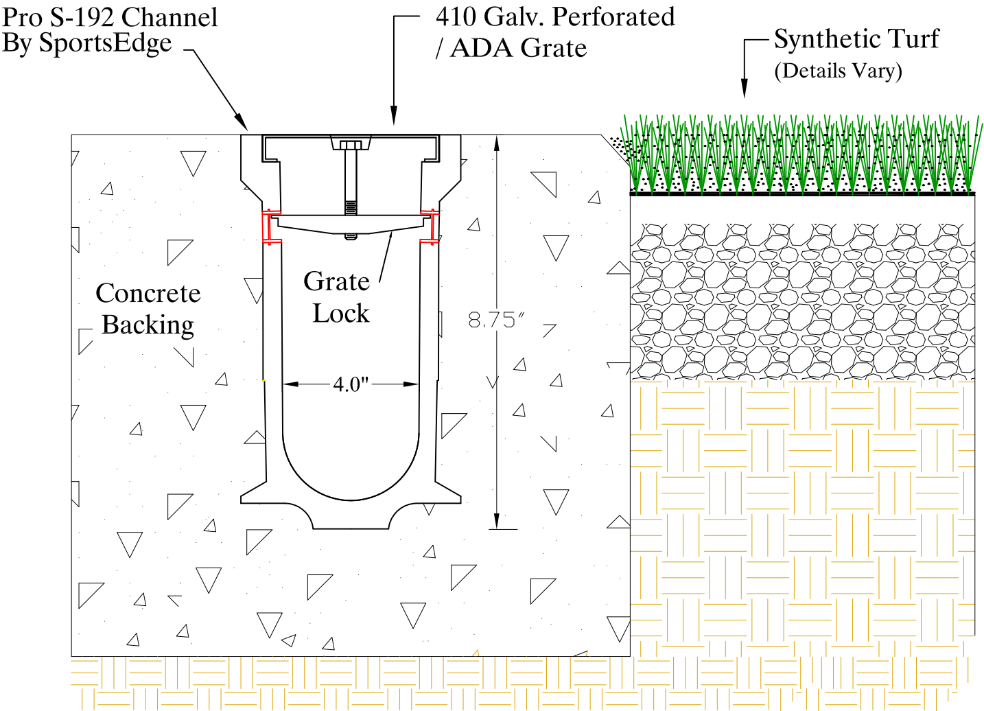
SportsEdge® Pro S-192 Channel Drain w/ #410 Galv. Perf. Grate
