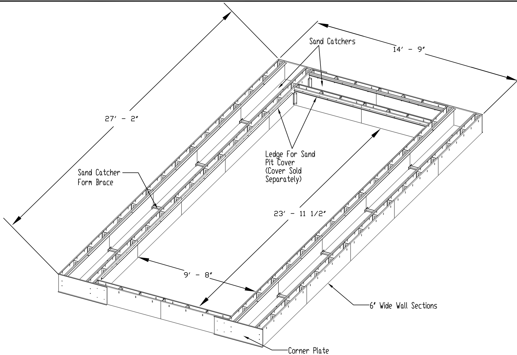
SportsEdge SEF44124 LONG / TRIPLE JUMP PIT FORM SYSTEM
