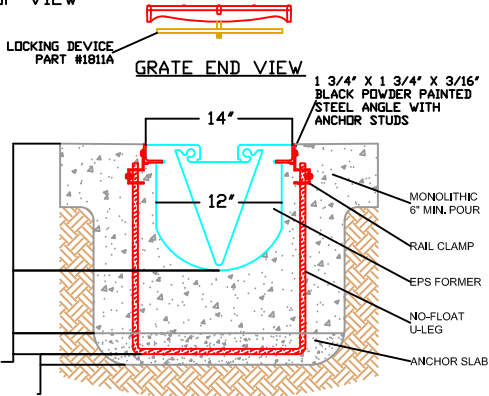
END CROSS SECTION VIEW
