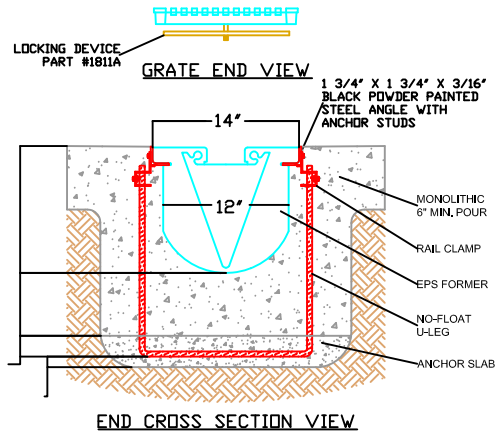
END CROSS SECTION VIEW
