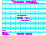
Option 2: 12.504G.F.B DUCTILE IRON ADA GRATE TOP VIEW
