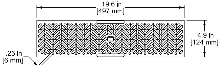
GRATE TOP VIEW (ROTATED 90°)
