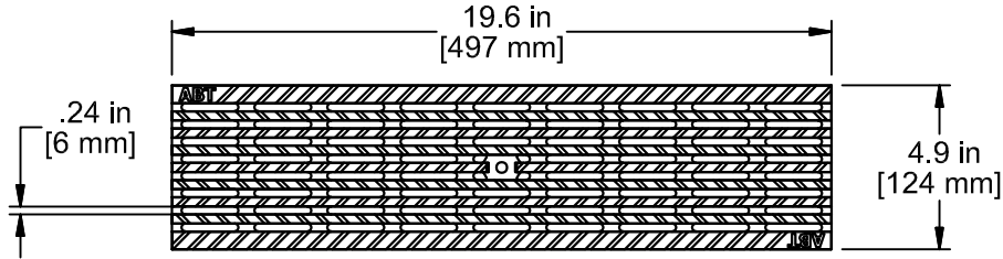
GRATE TOP VIEW (ROTATED 90°)
