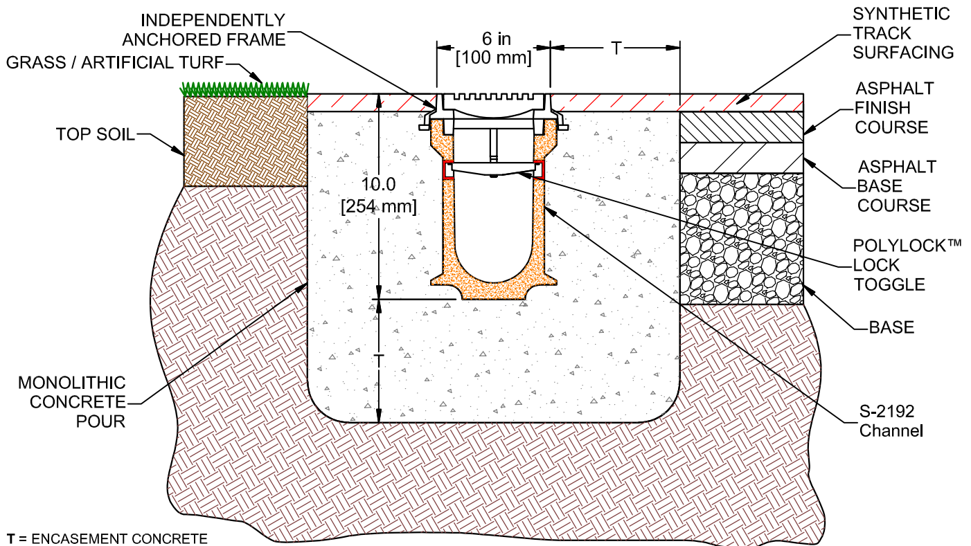
END CROSS SECTION VIEW
