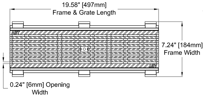
GRATE TOP VIEW (ROTATED 90°)
