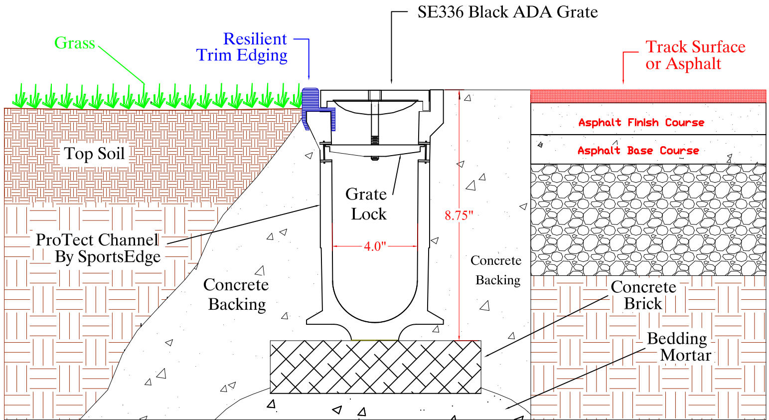
SportsEdge ProTect Channel - S192M Channel Drain Protective Trim Edge One Side NO SCALE
