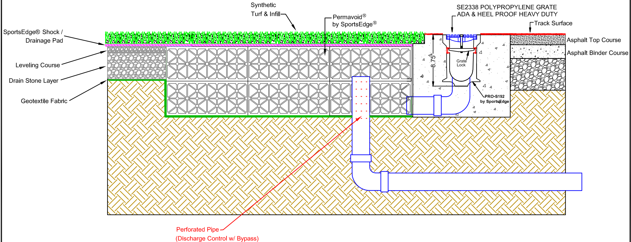
Plan View- SportsEdge PRO-S192 Surface Drain System w/ Shock/Drain Pad and Permavoid Water Control System
