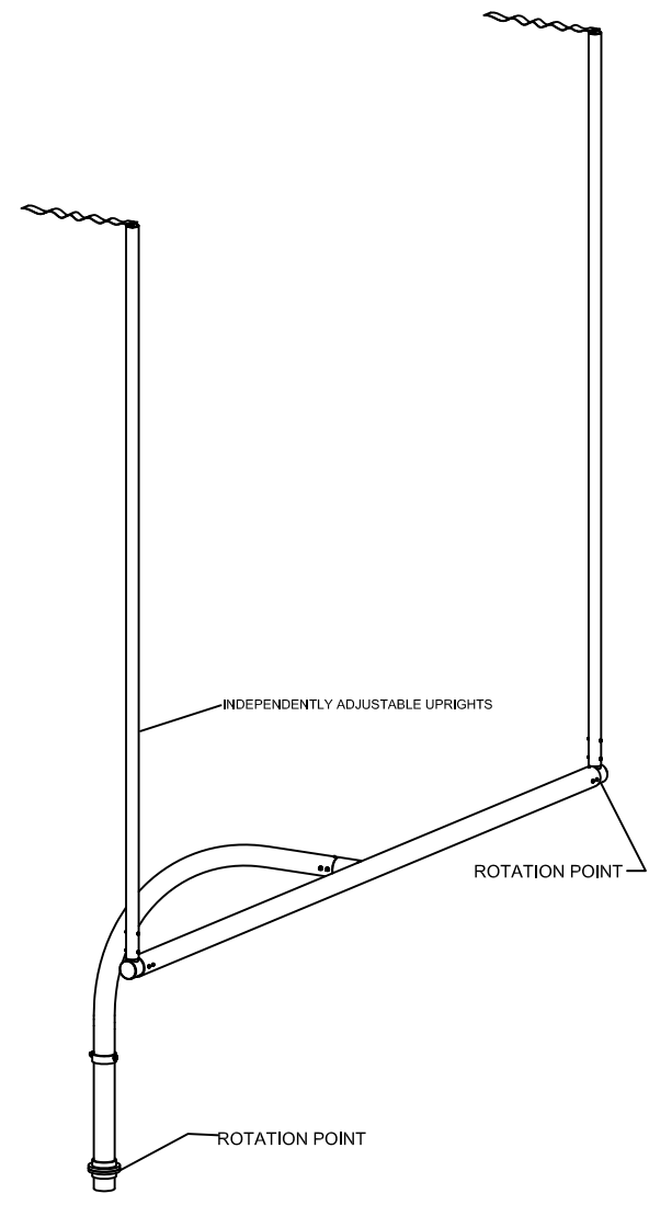
SEF305R ROTATABLE FOOTBALL GOAL POST Patent Pending
