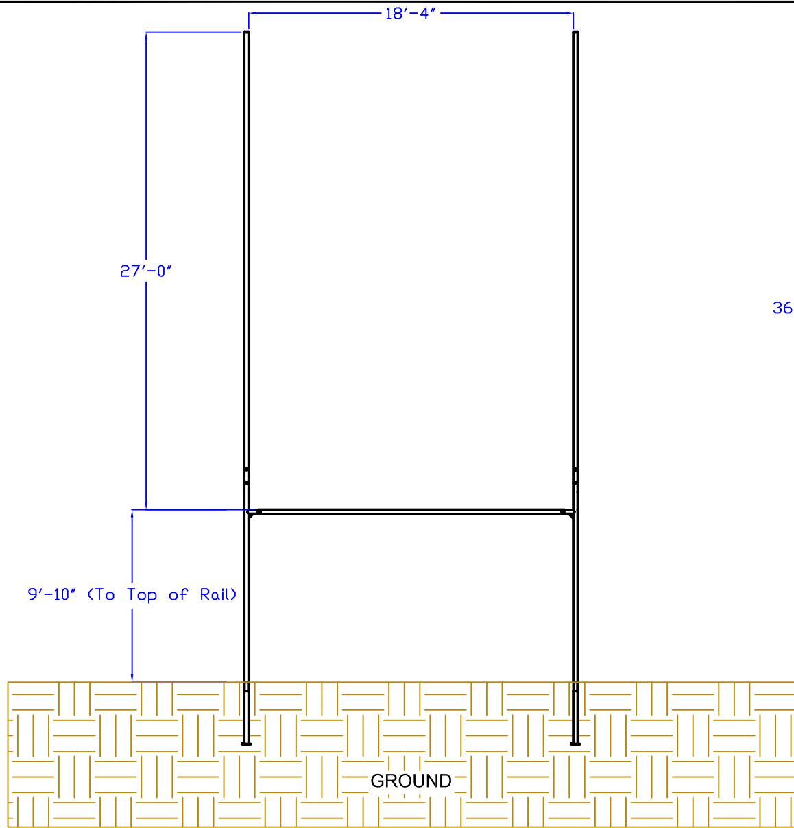
FRONT VIEW- Rugby Goals #SE2J102 as Supplied by SportsEdge
