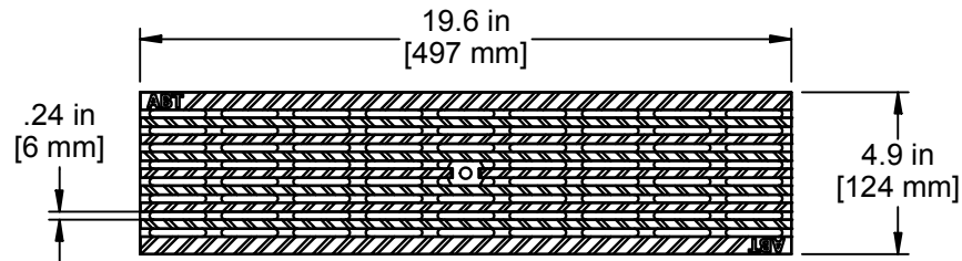
GRATE TOP VIEW (ROTATED 90°)
