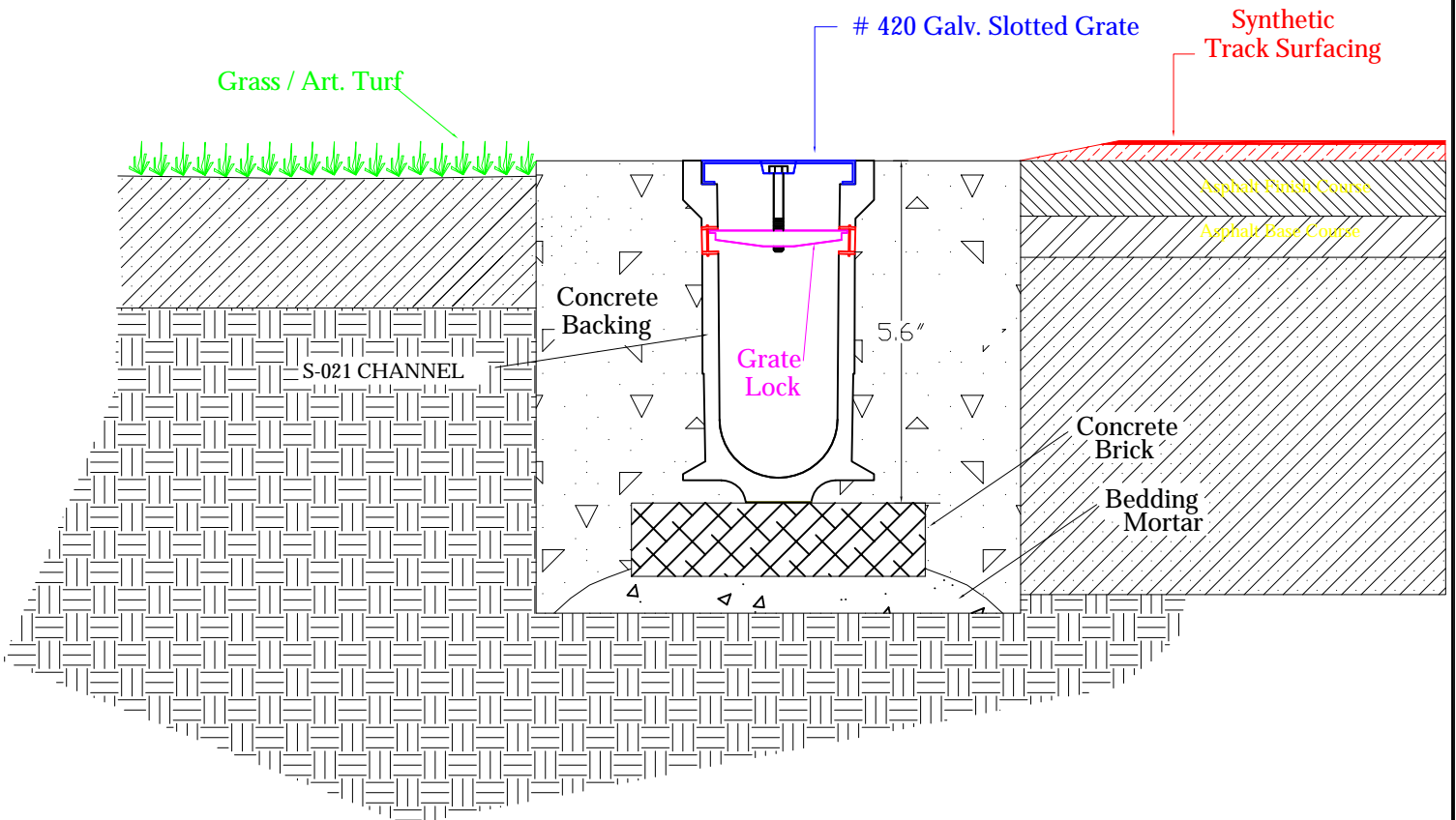
Section- SportsEdge Pro-S Channel #S-021 Typ. Detail- No Scale
