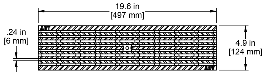
GRATE TOP VIEW (ROTATED 90°)
