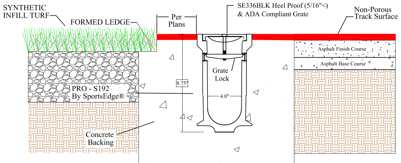
SPORTSEGE® PRO-S192 Channel Drain Formed Ledge / Syn. Turf - Non-Porous Track Surface
