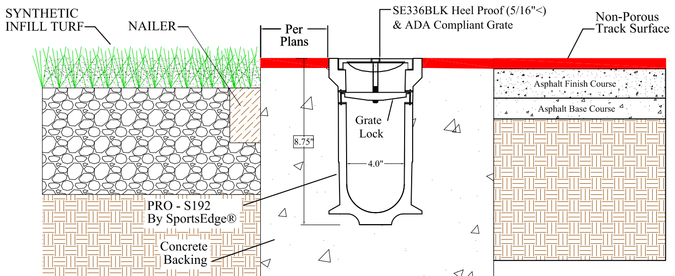
SPORTSEGE® PRO-S192 Channel Drain Wood Nailer / Syn. Turf - Non-Porous Track Surface
