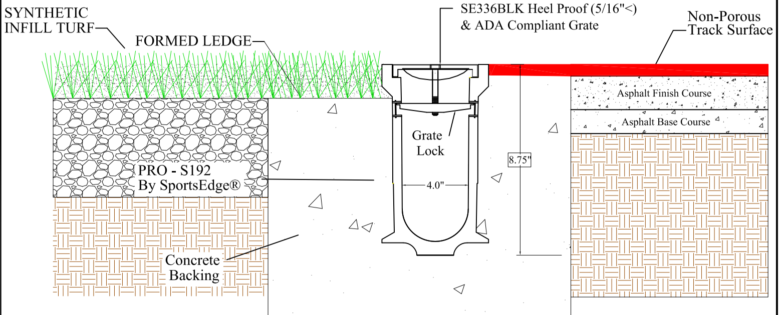
SPORTSEdge® PRO-S192 Channel Drain Low Ledge Syn. Turf - Non-Porous Track Surface
