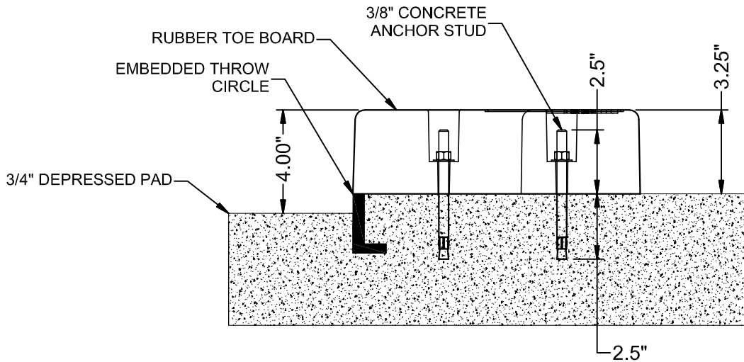
END VIEW
