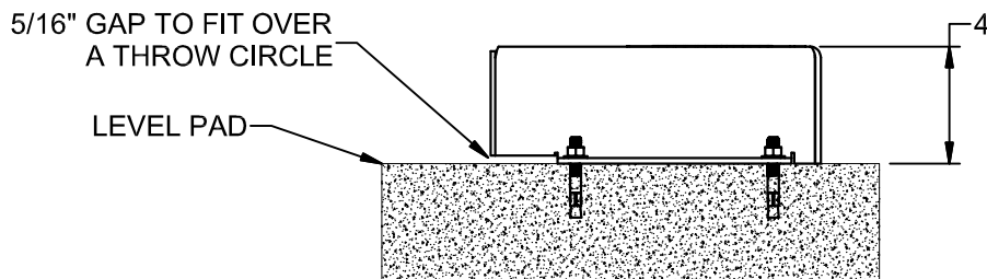
END VIEW
