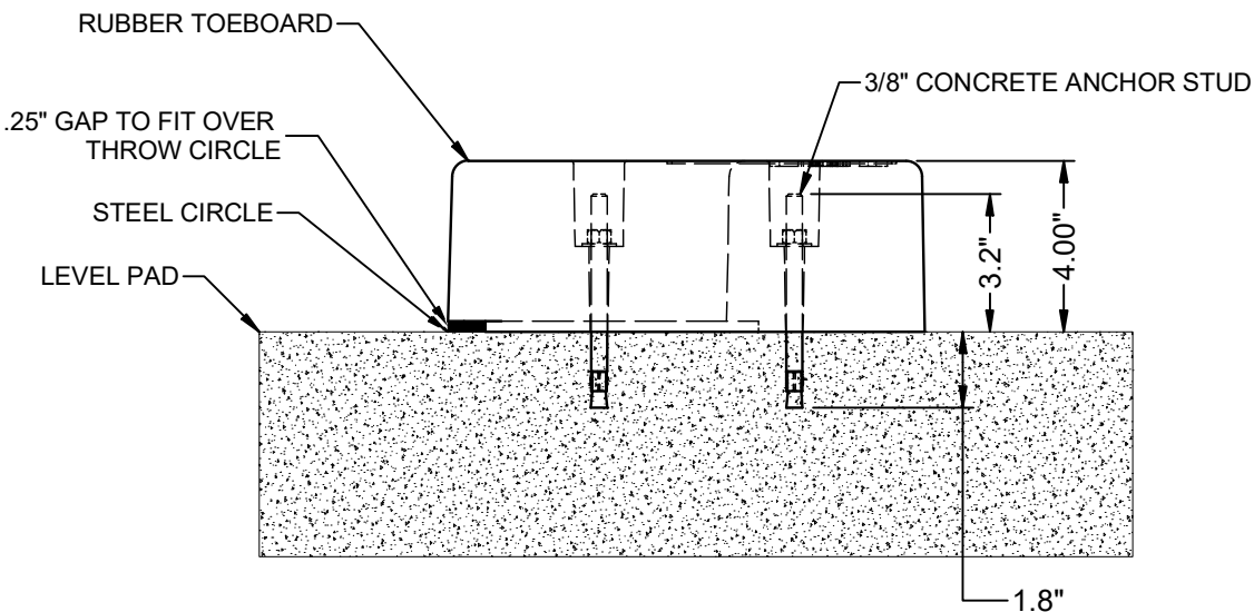
END VIEW
