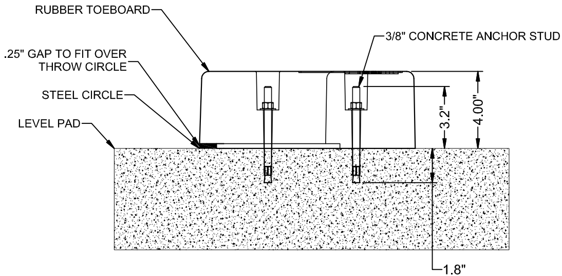
END VIEW
