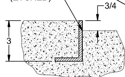
SECTION A-A AFTER INSTALLATION
