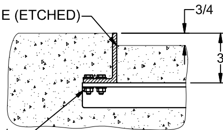
SECTION B-B AFTER INSTALLATION
