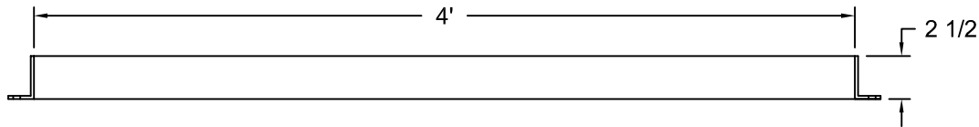
SIDE VIEW
